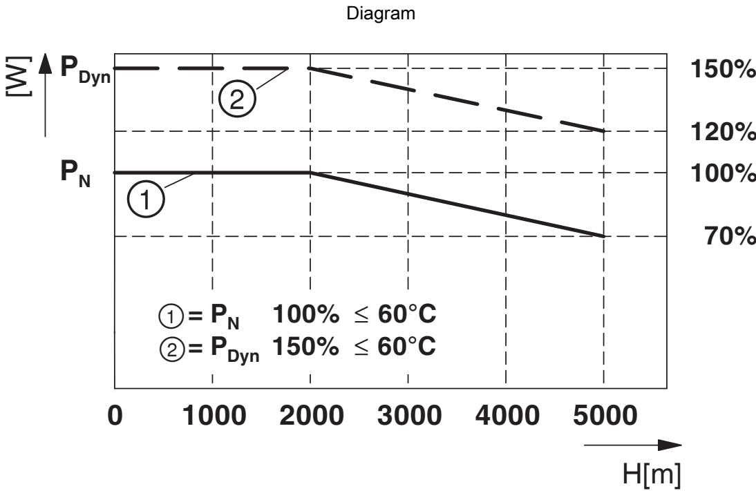
Altitude-dependent derating
